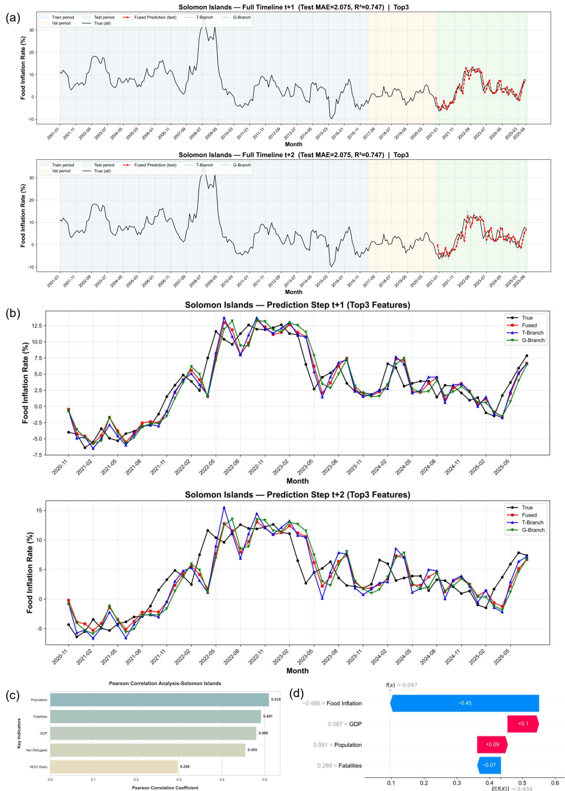
Multidimensional Evaluation and Attribution Analysis of Food Inflation Forecast in Solomon Islands. (a) Overview of the total cycle prediction and fitting, (b) Multi-step Short-Term Forecast Comparison Chart, (c) Pearson correlation analysis of macroeconomic drivers, (d) SHAP-based explanation of feature contributions for a specific prediction instance.
